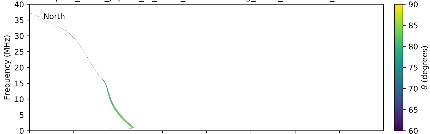
expres_earth_jupiter_io_isaac_lossc-wid1deg_3kev_20071230_v01.cdf
