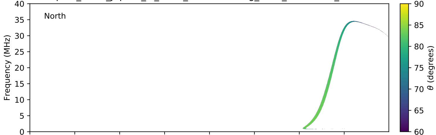
expres_earth_jupiter_io_isaac_lossc-wid1deg_3kev_20071227_v01.cdf
