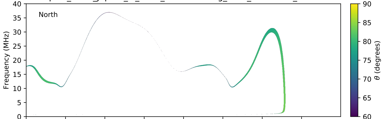
expres_earth_jupiter_io_isaac_lossc-wid1deg_3kev_20071226_v01.cdf
