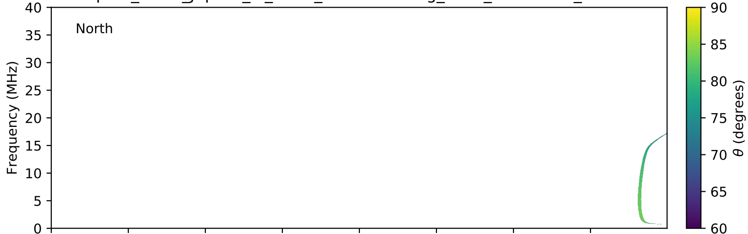
expres_earth_jupiter_io_isaac_lossc-wid1deg_3kev_20071225_v01.cdf
