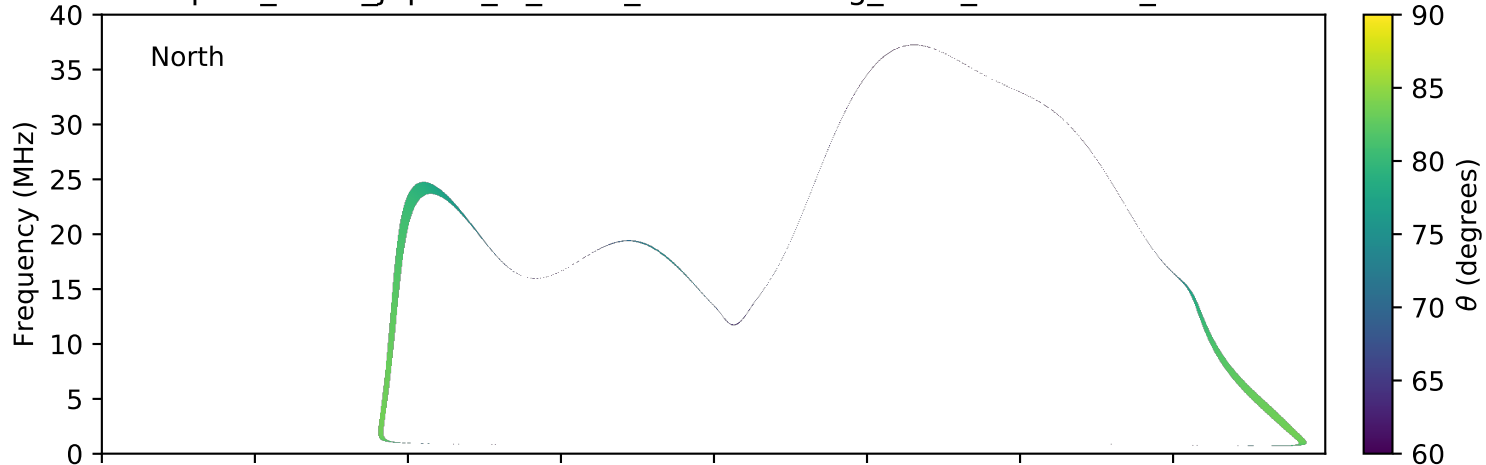
expres_earth_jupiter_io_isaac_lossc-wid1deg_3kev_20071224_v01.cdf
