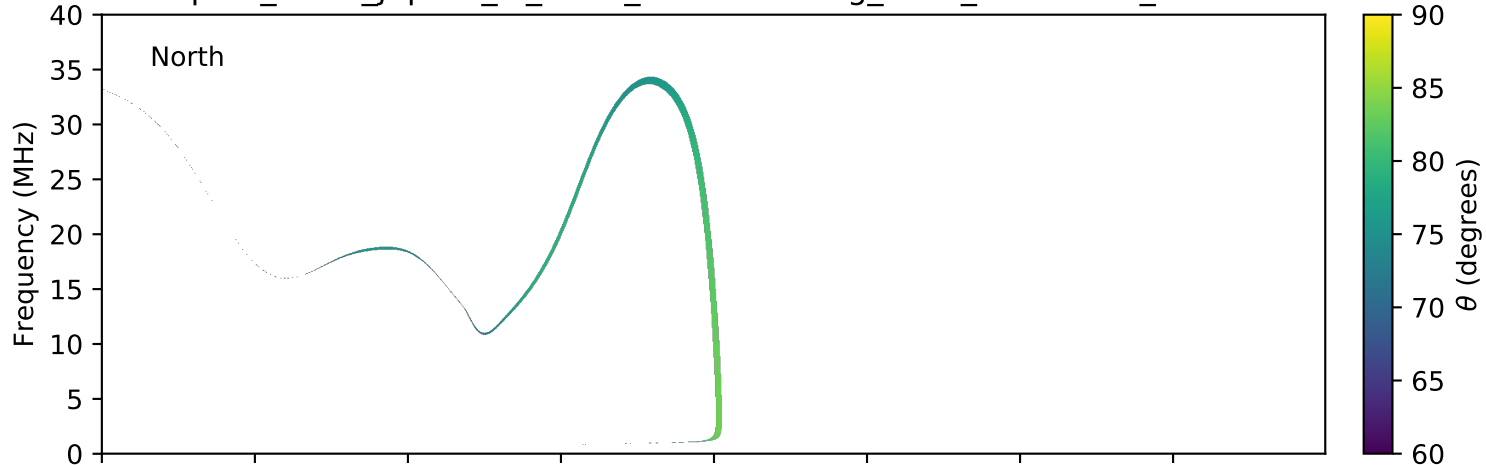
expres_earth_jupiter_io_isaac_lossc-wid1deg_3kev_20071221_v01.cdf
