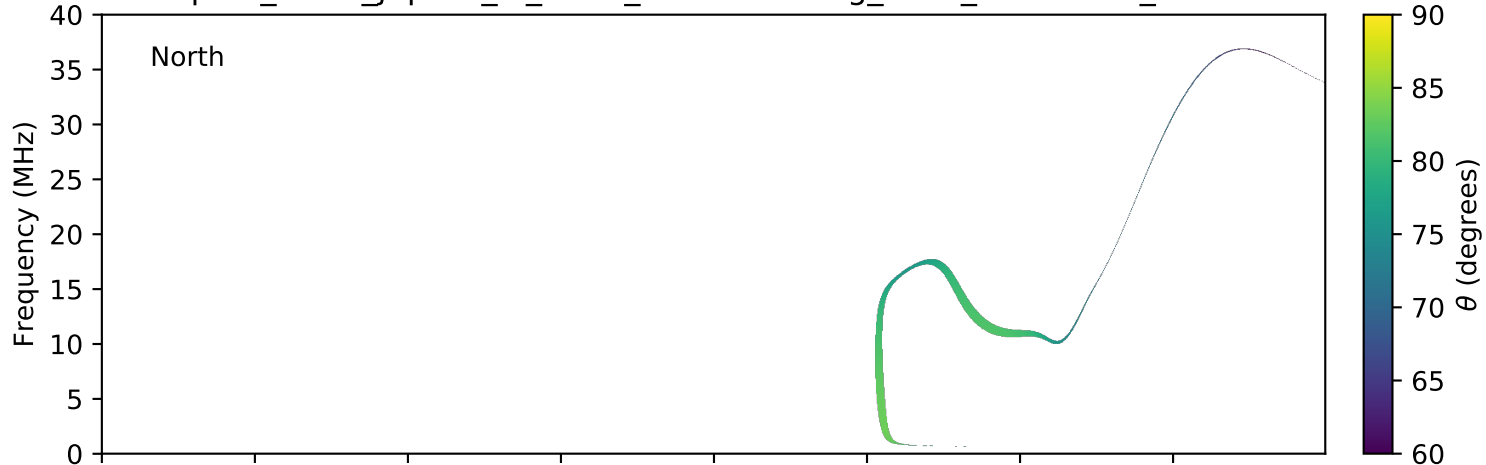
expres_earth_jupiter_io_isaac_lossc-wid1deg_3kev_20071220_v01.cdf
