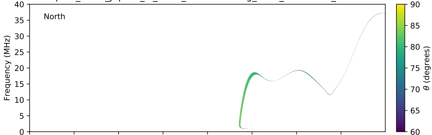
expres_earth_jupiter_io_isaac_lossc-wid1deg_3kev_20071213_v01.cdf
