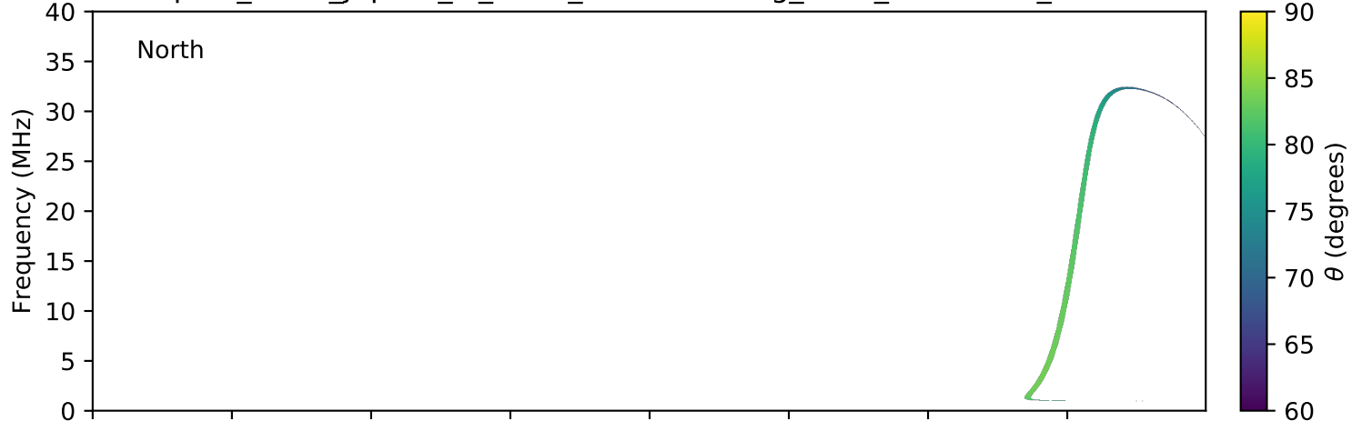
expres_earth_jupiter_io_isaac_lossc-wid1deg_3kev_20071211_v01.cdf
