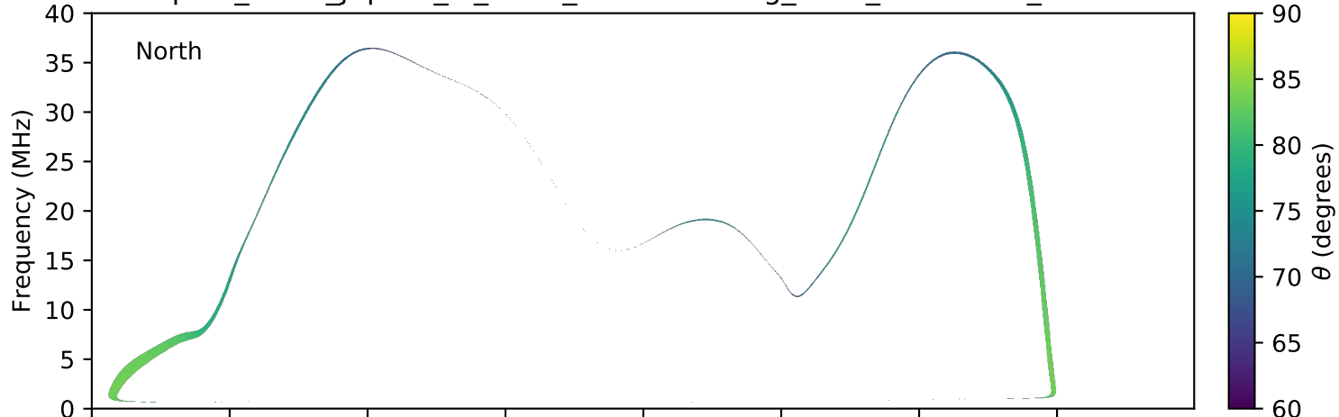
expres_earth_jupiter_io_isaac_lossc-wid1deg_3kev_20071210_v01.cdf
