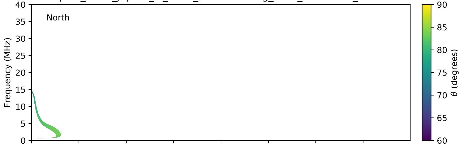
expres_earth_jupiter_io_isaac_lossc-wid1deg_3kev_20071209_v01.cdf
