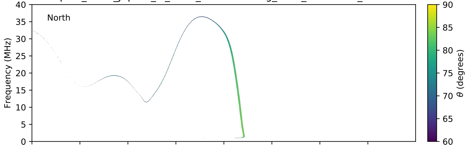
expres_earth_jupiter_io_isaac_lossc-wid1deg_3kev_20071205_v01.cdf
