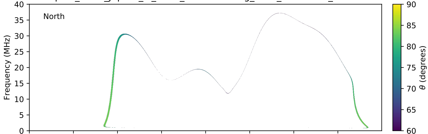
expres_earth_jupiter_io_isaac_lossc-wid1deg_3kev_20071201_v01.cdf
