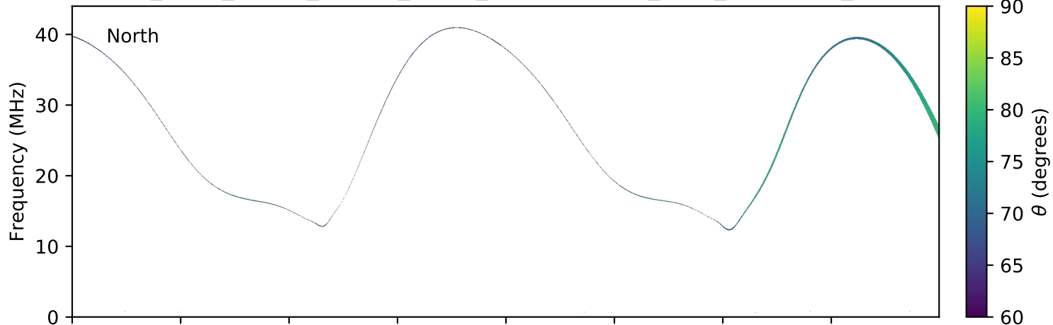
expres_earth_jupiter_europa_jrm09_lossc-wid1deg_3kev_20071228_v01.cdf
