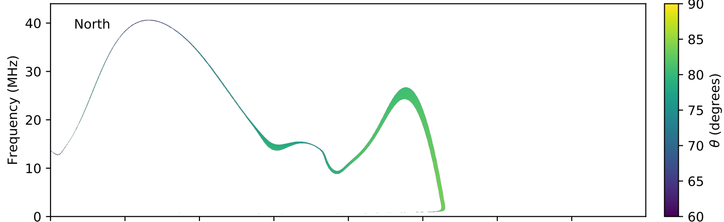
expres_earth_jupiter_europa_jrm09_lossc-wid1deg_3kev_20071225_v01.cdf
