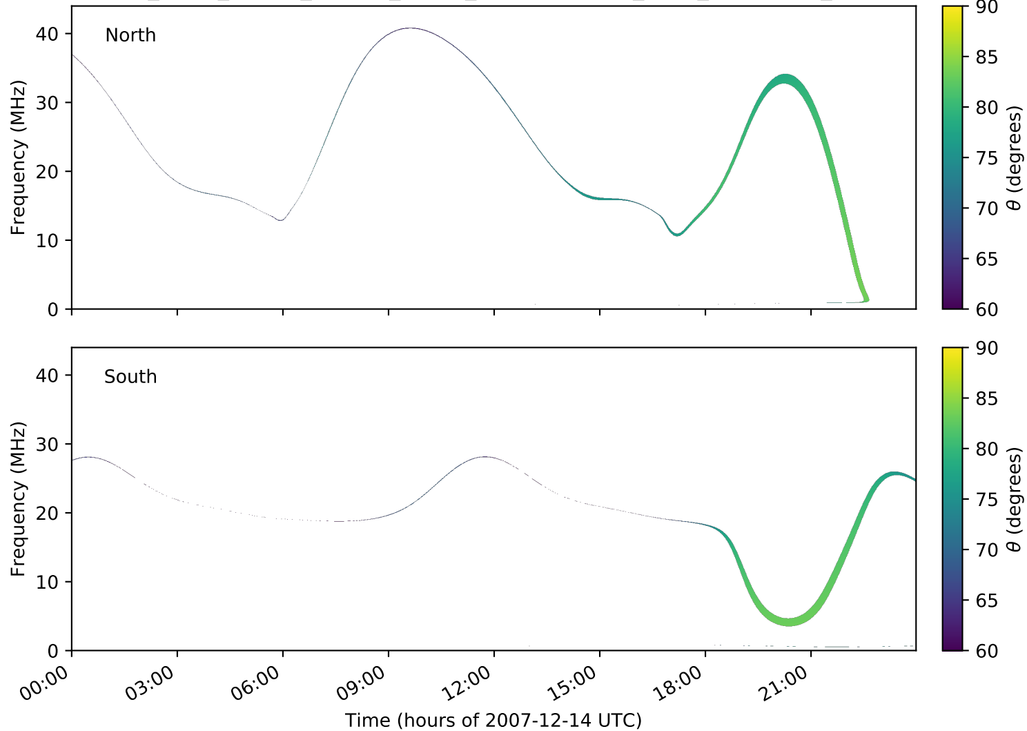
expres_earth_jupiter_europa_jrm09_lossc-wid1deg_3kev_20071214_v01.cdf
