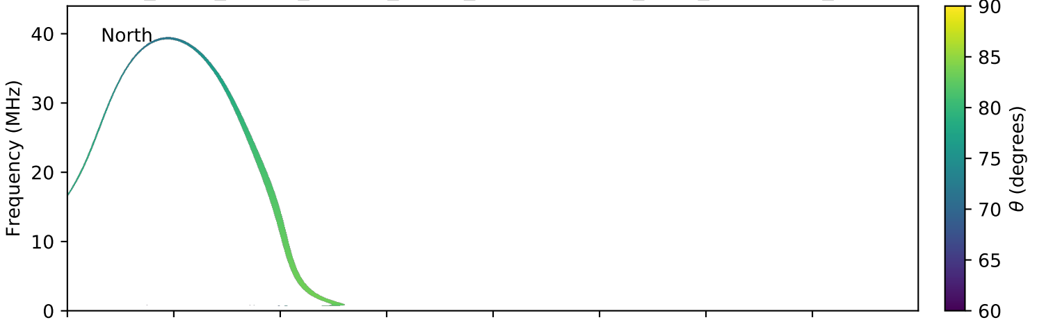
expres_earth_jupiter_europa_jrm09_lossc-wid1deg_3kev_20071211_v01.cdf
