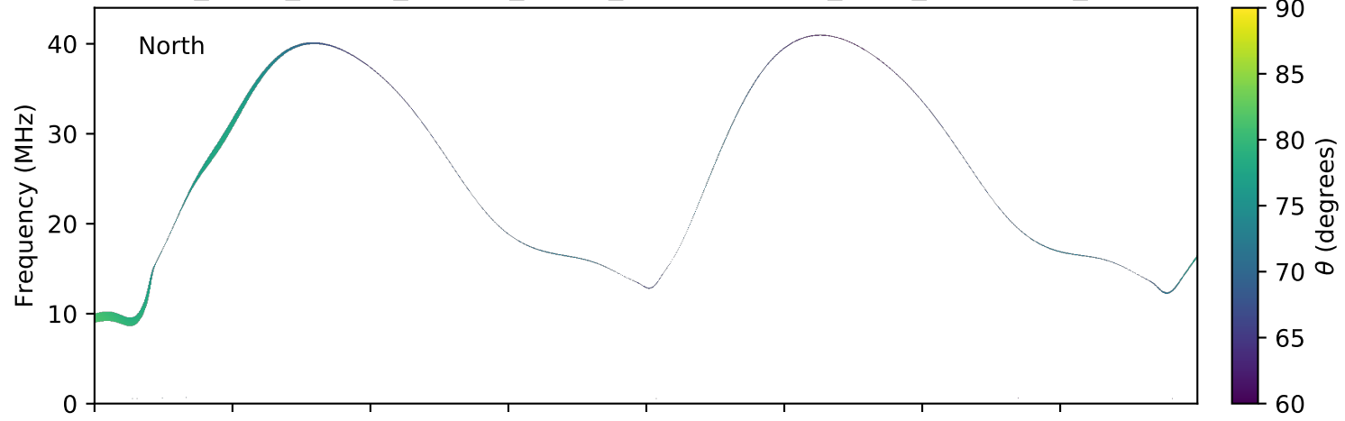
expres_earth_jupiter_europa_jrm09_lossc-wid1deg_3kev_20071210_v01.cdf
