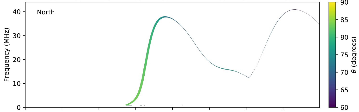
expres_earth_jupiter_europa_jrm09_lossc-wid1deg_3kev_20071206_v01.cdf
