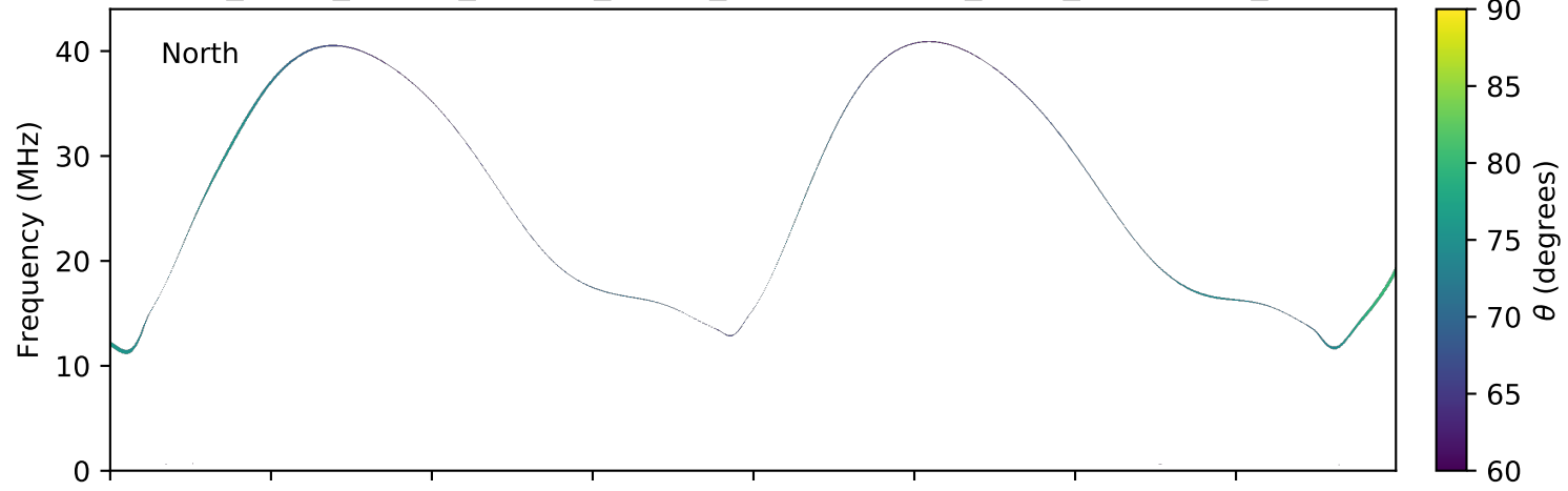
expres_earth_jupiter_europa_jrm09_lossc-wid1deg_3kev_20071203_v01.cdf
