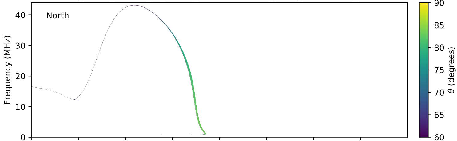
expres_earth_jupiter_io_jrm09_lossc-wid1deg_3kev_20071128_v01.cdf
