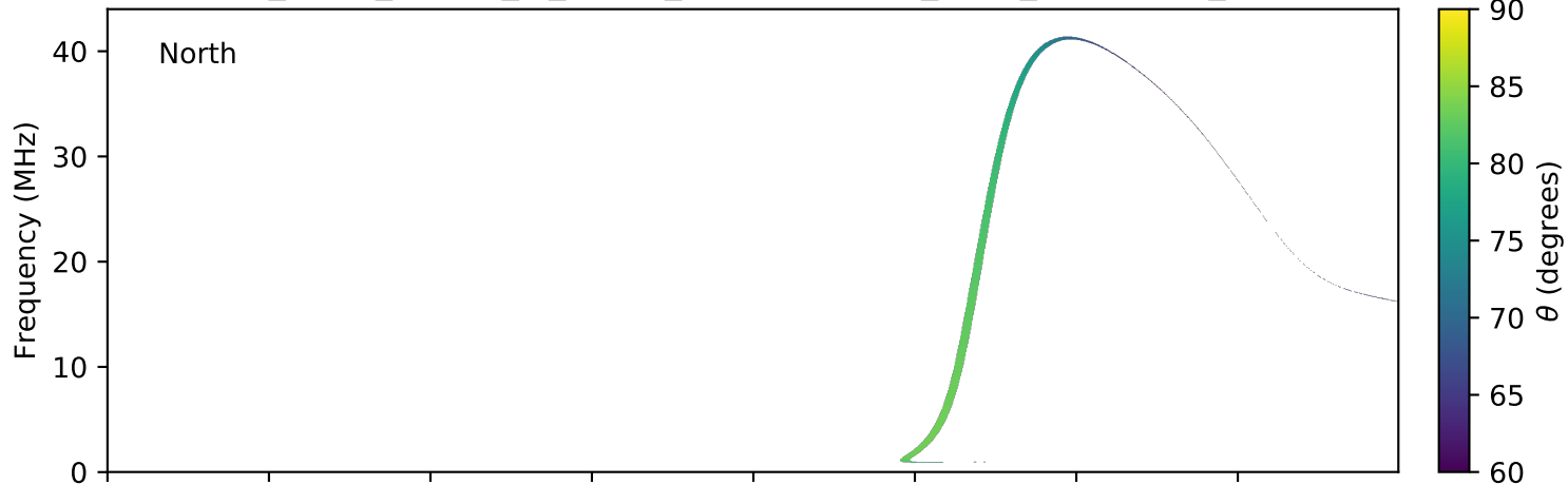
expres_earth_jupiter_io_jrm09_lossc-wid1deg_3kev_20071120_v01.cdf
