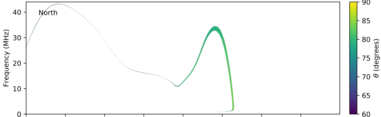
expres_earth_jupiter_io_jrm09_lossc-wid1deg_3kev_20071119_v01.cdf
