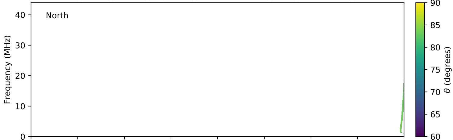
expres_earth_jupiter_io_jrm09_lossc-wid1deg_3kev_20071109_v01.cdf
