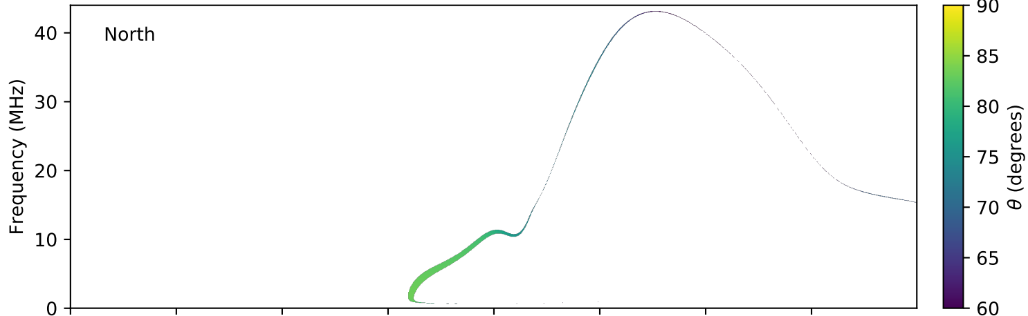
expres_earth_jupiter_io_jrm09_lossc-wid1deg_3kev_20071106_v01.cdf
