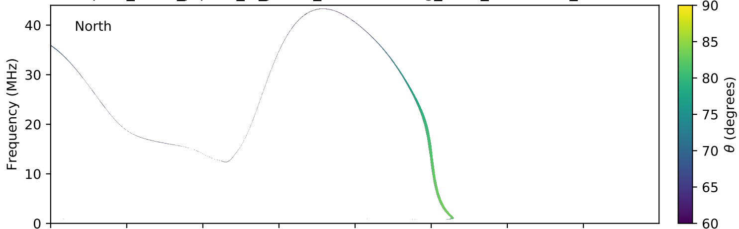
expres_earth_jupiter_io_jrm09_lossc-wid1deg_3kev_20071103_v01.cdf
