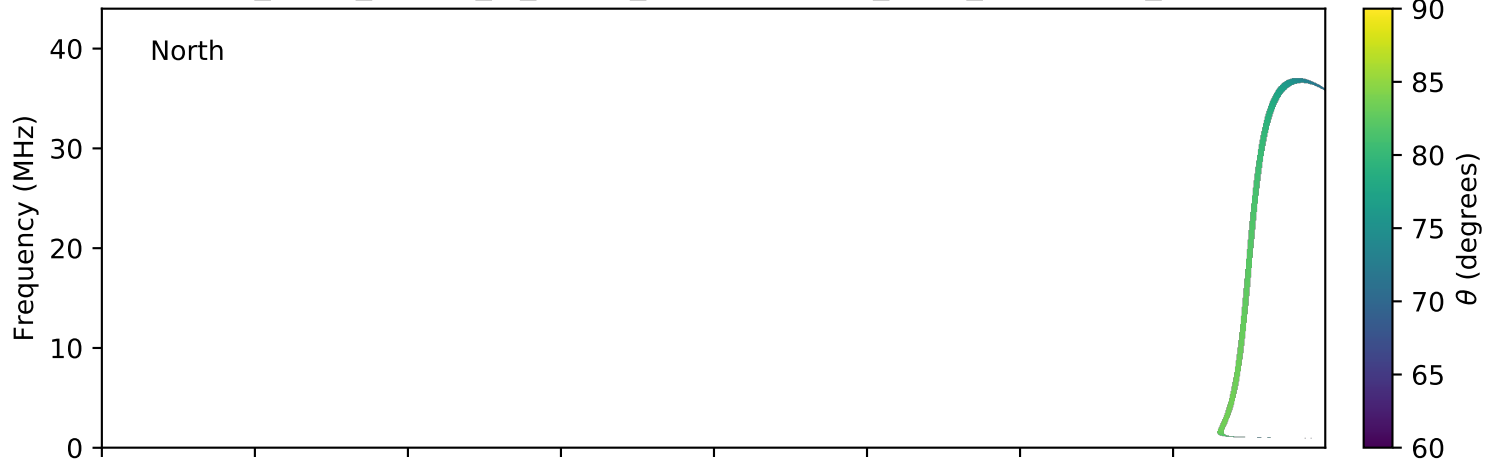
expres_earth_jupiter_io_jrm09_lossc-wid1deg_3kev_20071102_v01.cdf
