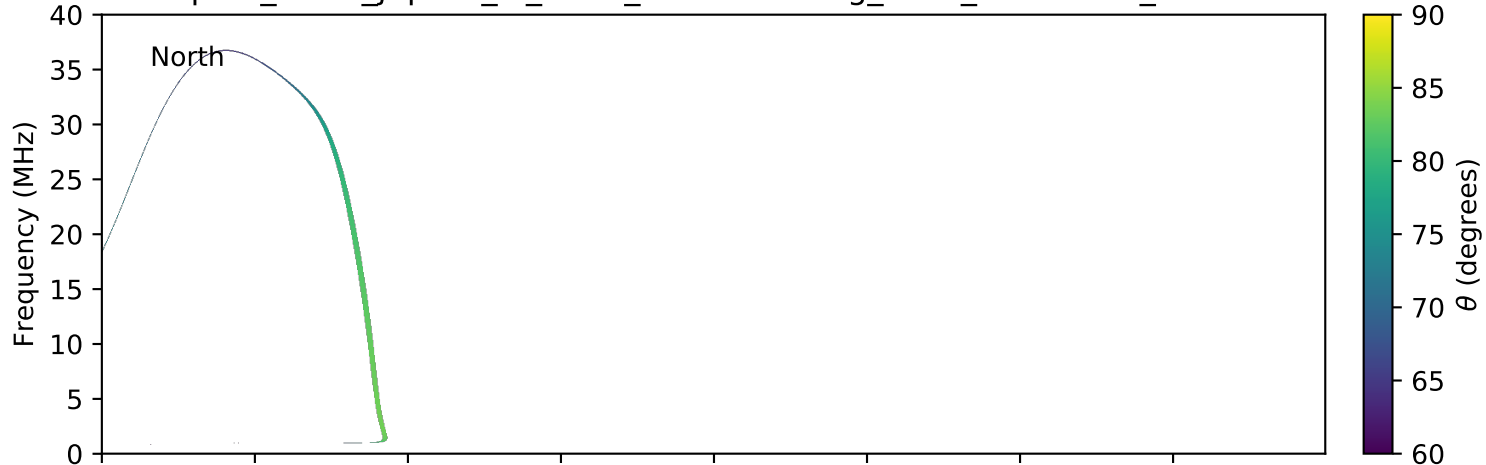
expres_earth_jupiter_io_isaac_lossc-wid1deg_3kev_20071130_v01.cdf
