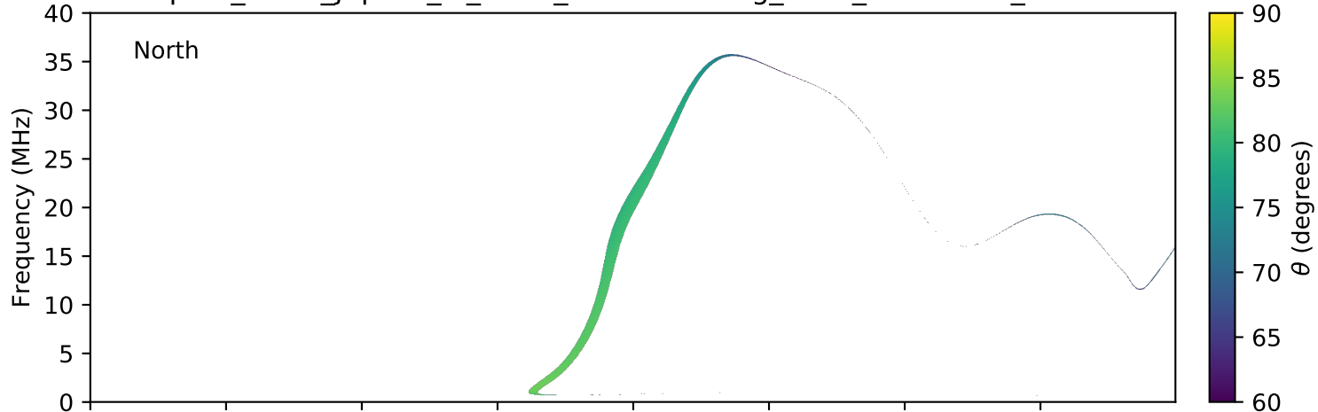
expres_earth_jupiter_io_isaac_lossc-wid1deg_3kev_20071129_v01.cdf
