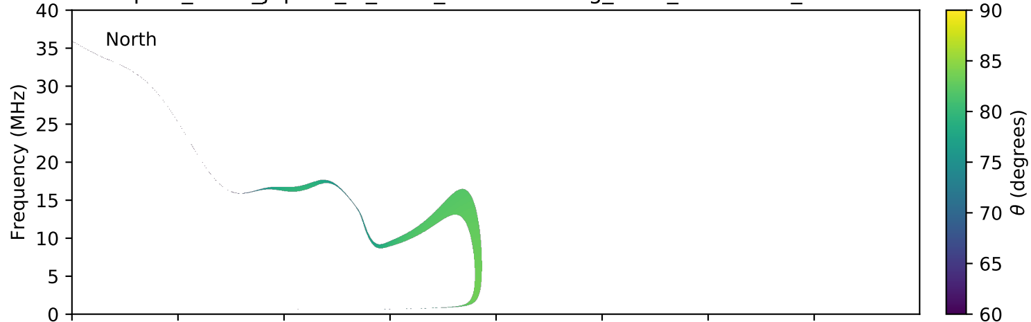
expres_earth_jupiter_io_isaac_lossc-wid1deg_3kev_20071128_v01.cdf
