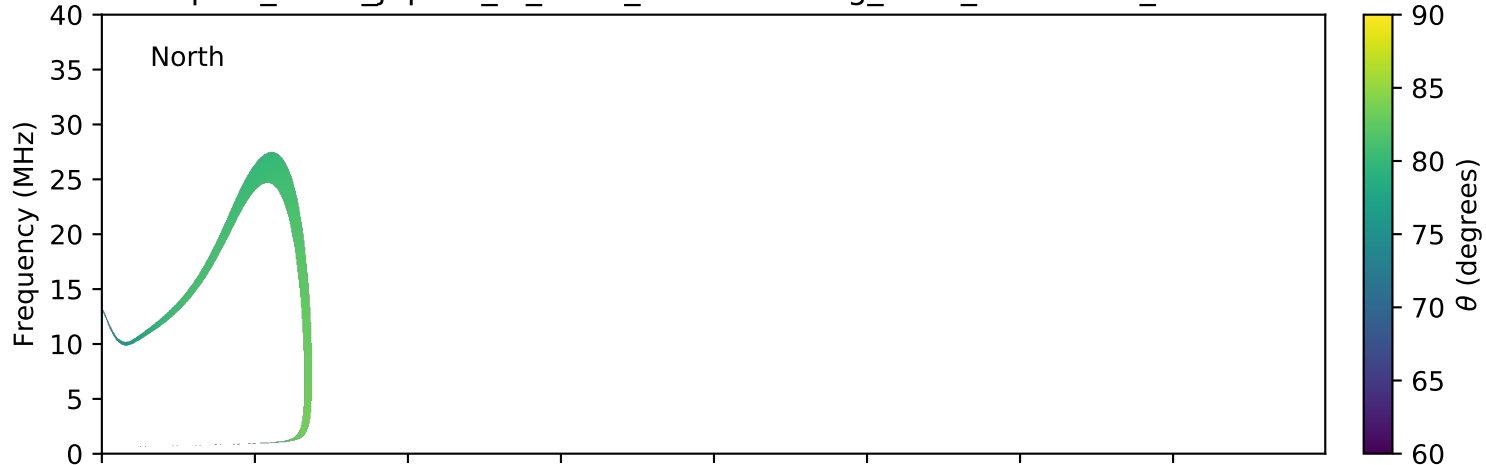
expres_earth_jupiter_io_isaac_lossc-wid1deg_3kev_20071123_v01.cdf
