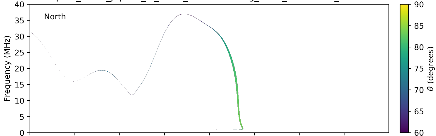
expres_earth_jupiter_io_isaac_lossc-wid1deg_3kev_20071119_v01.cdf
