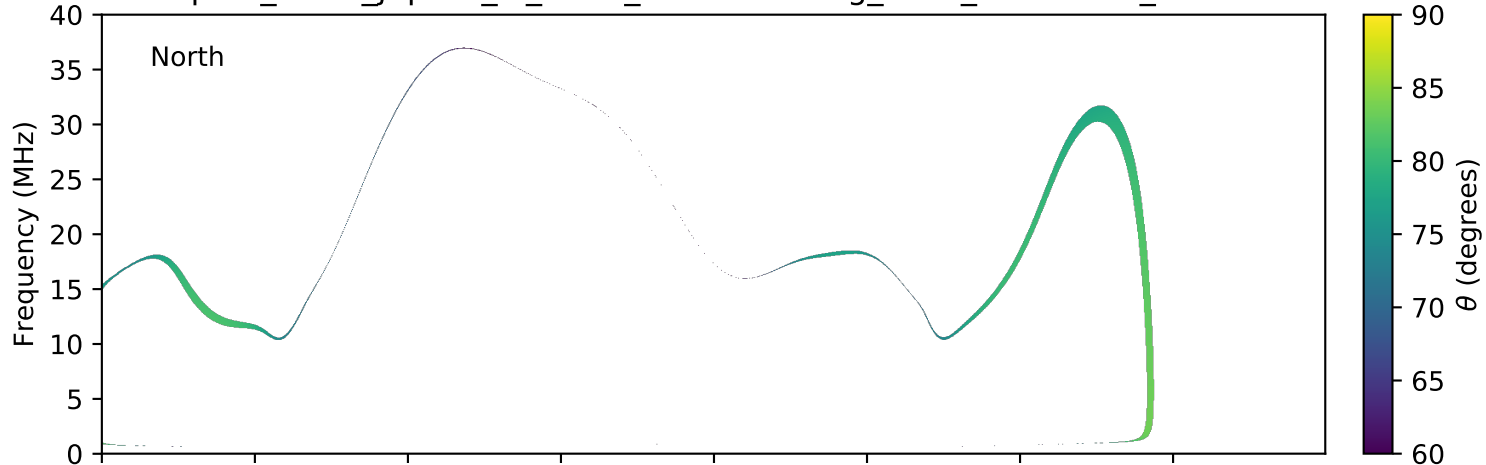
expres_earth_jupiter_io_isaac_lossc-wid1deg_3kev_20071117_v01.cdf
