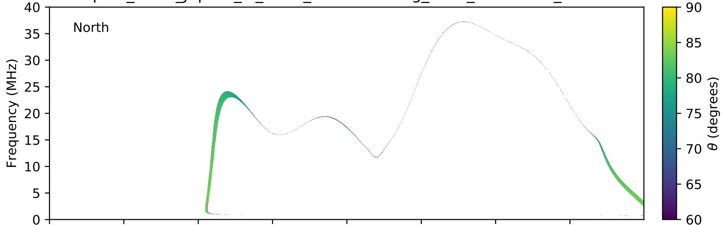
expres_earth_jupiter_io_isaac_lossc-wid1deg_3kev_20071115_v01.cdf
