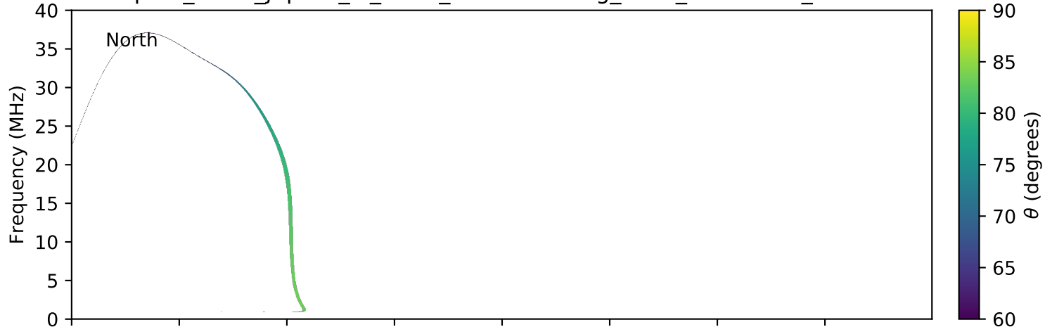
expres_earth_jupiter_io_isaac_lossc-wid1deg_3kev_20071114_v01.cdf
