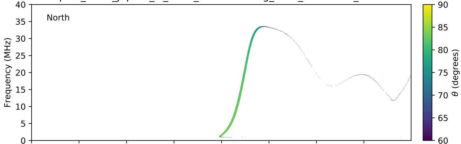
expres_earth_jupiter_io_isaac_lossc-wid1deg_3kev_20071113_v01.cdf
