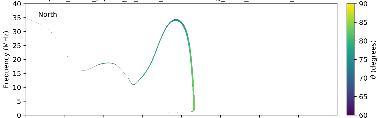
expres_earth_jupiter_io_isaac_lossc-wid1deg_3kev_20071112_v01.cdf
