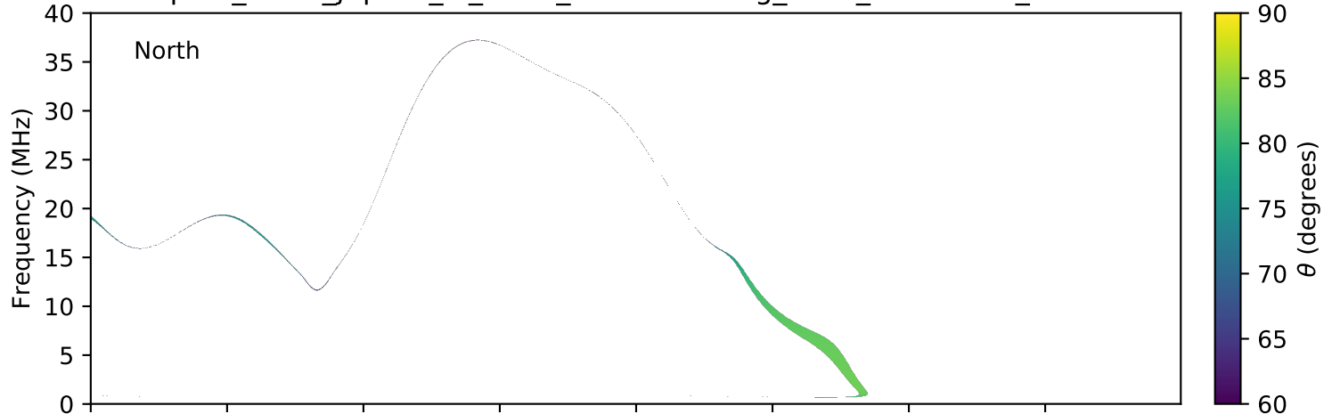
expres_earth_jupiter_io_isaac_lossc-wid1deg_3kev_20071110_v01.cdf
