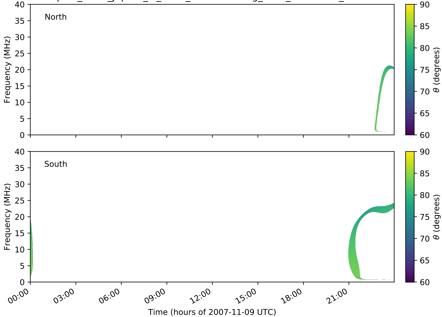
expres_earth_jupiter_io_isaac_lossc-wid1deg_3kev_20071109_v01.cdf
