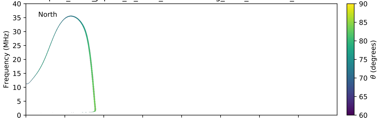
expres_earth_jupiter_io_isaac_lossc-wid1deg_3kev_20071107_v01.cdf
