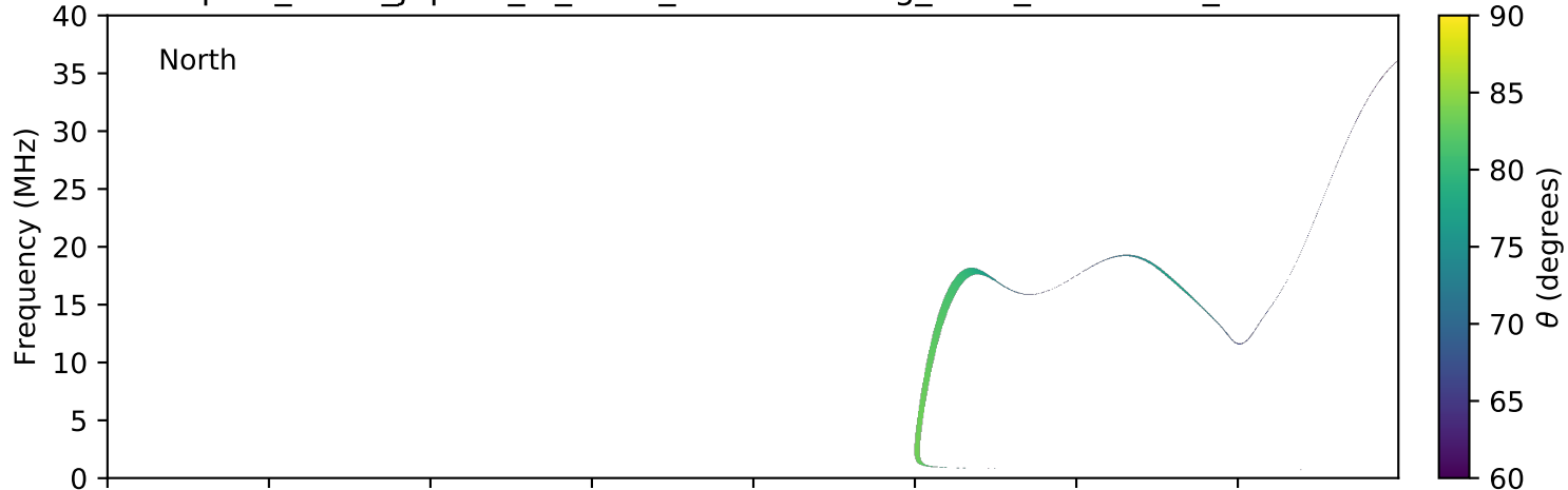
expres_earth_jupiter_io_isaac_lossc-wid1deg_3kev_20071104_v01.cdf
