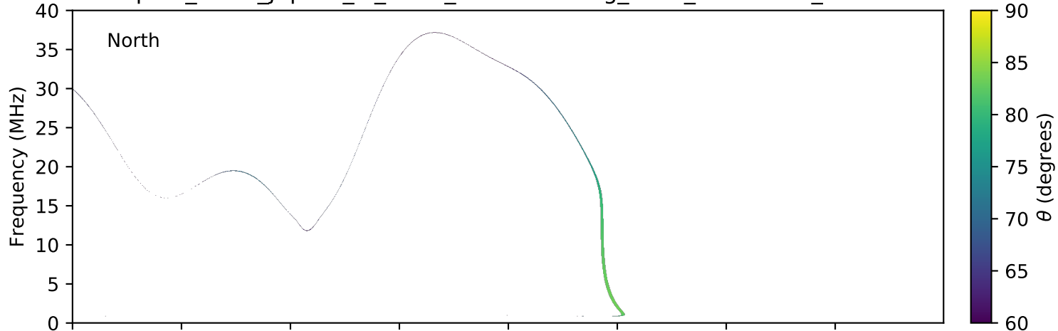
expres_earth_jupiter_io_isaac_lossc-wid1deg_3kev_20071103_v01.cdf
