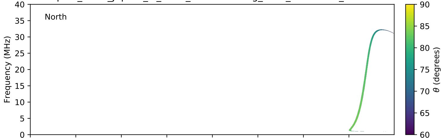
expres_earth_jupiter_io_isaac_lossc-wid1deg_3kev_20071102_v01.cdf
