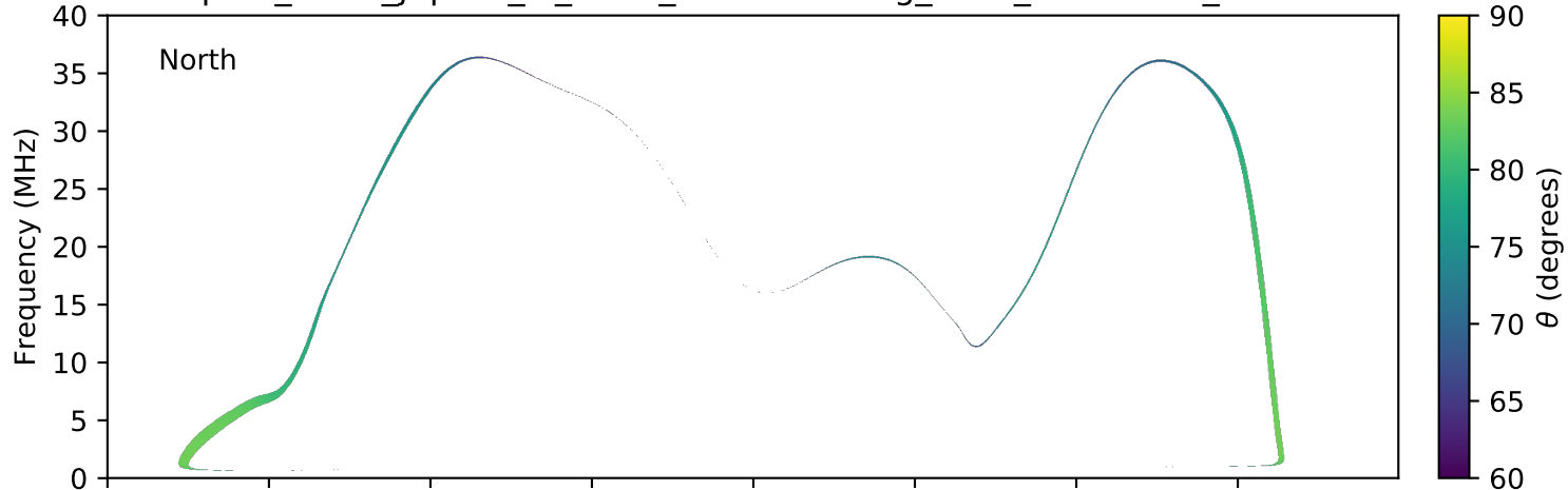
expres_earth_jupiter_io_isaac_lossc-wid1deg_3kev_20071101_v01.cdf
