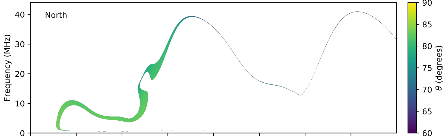
expres_earth_jupiter_europa_jrm09_lossc-wid1deg_3kev_20071129_v01.cdf
