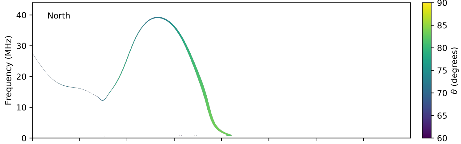
expres_earth_jupiter_europa_jrm09_lossc-wid1deg_3kev_20071123_v01.cdf
