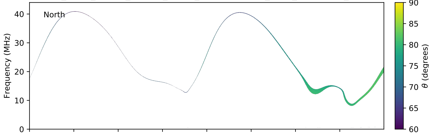
expres_earth_jupiter_europa_jrm09_lossc-wid1deg_3kev_20071119_v01.cdf
