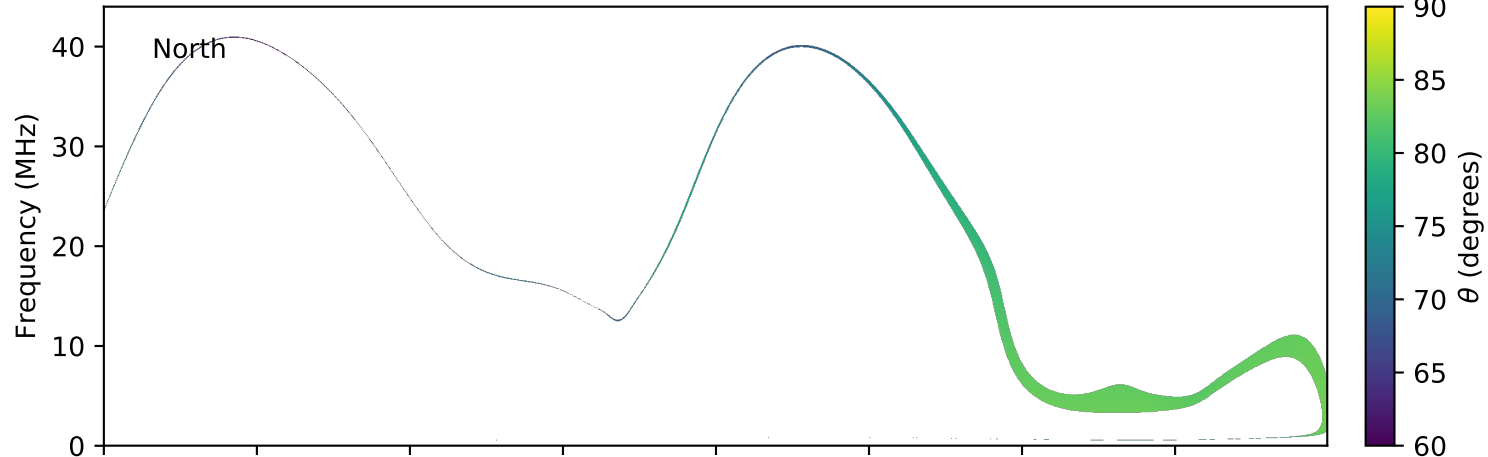
expres_earth_jupiter_europa_jrm09_lossc-wid1deg_3kev_20071112_v01.cdf
