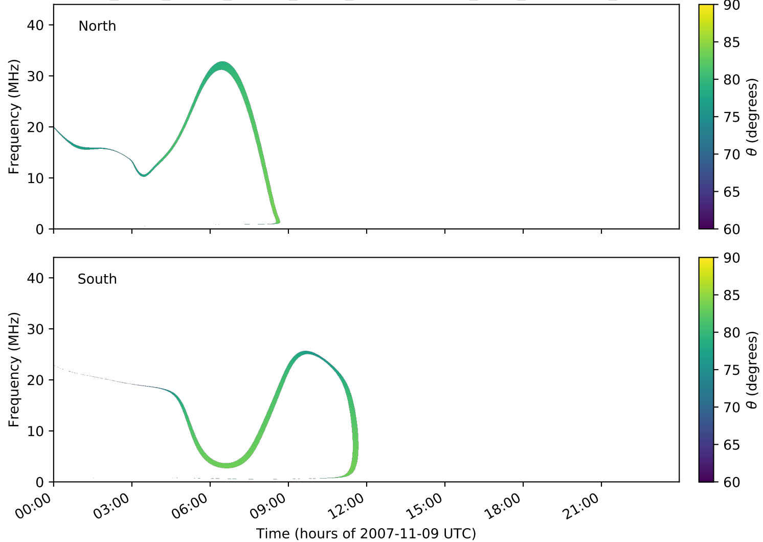
expres_earth_jupiter_europa_jrm09_lossc-wid1deg_3kev_20071109_v01.cdf
