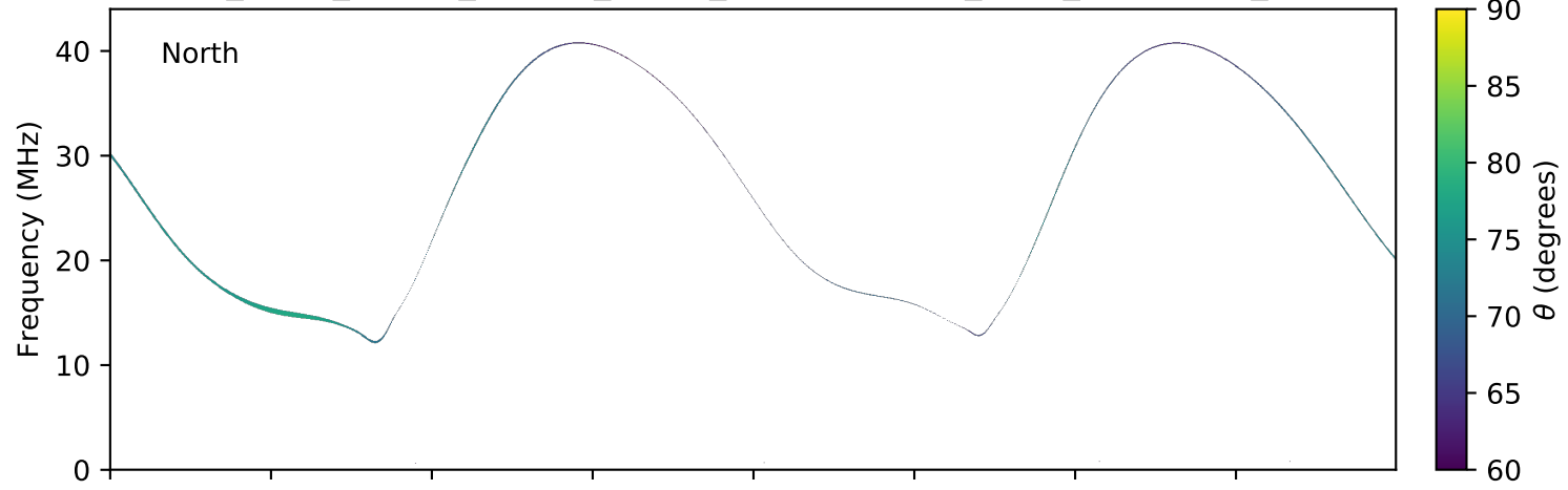
expres_earth_jupiter_europa_jrm09_lossc-wid1deg_3kev_20071108_v01.cdf
